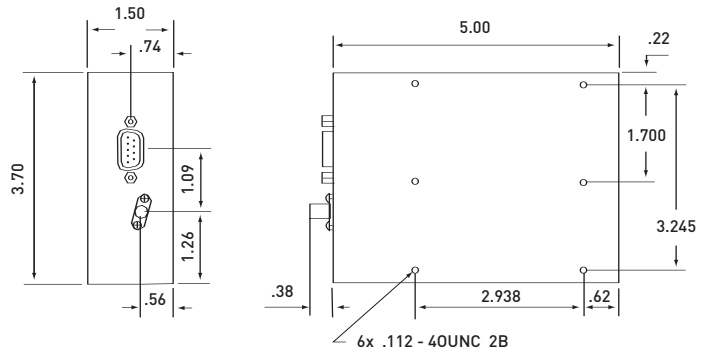
Outline Dimensions
